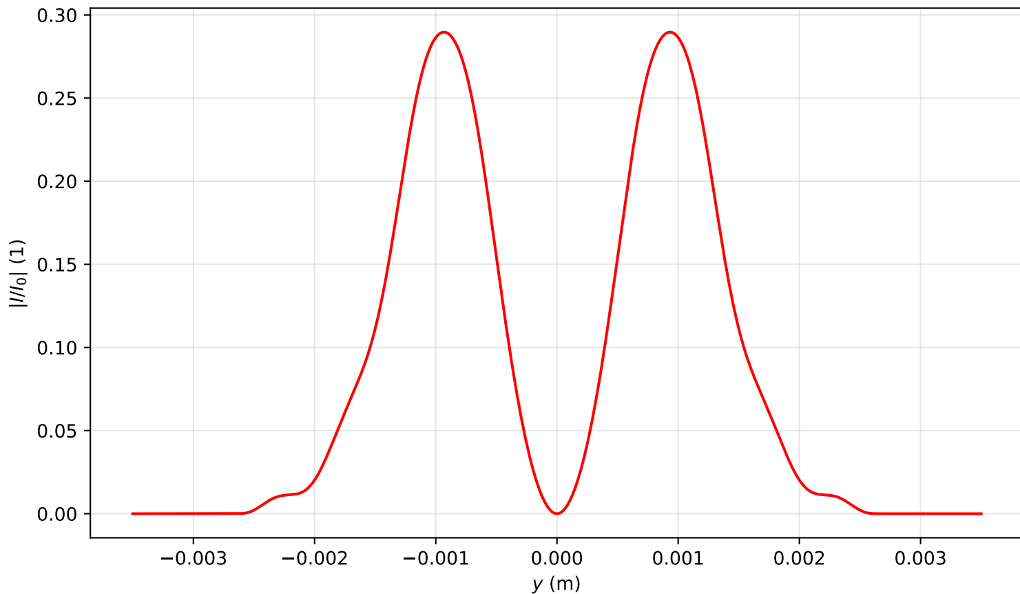
Intensity profile I(x=0, y, z=3.582)/I_0 , P_{in}=2.0P_{cr} , artificial time
